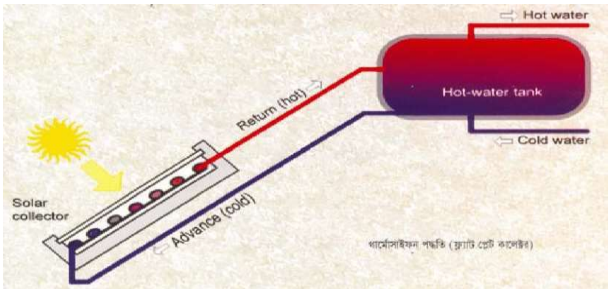
Figure 1: Thermosyphon solar heating system (Eschenbach, 2015)
